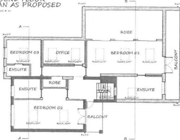
FIRST FLOOR PLAN AS PROPOSED
