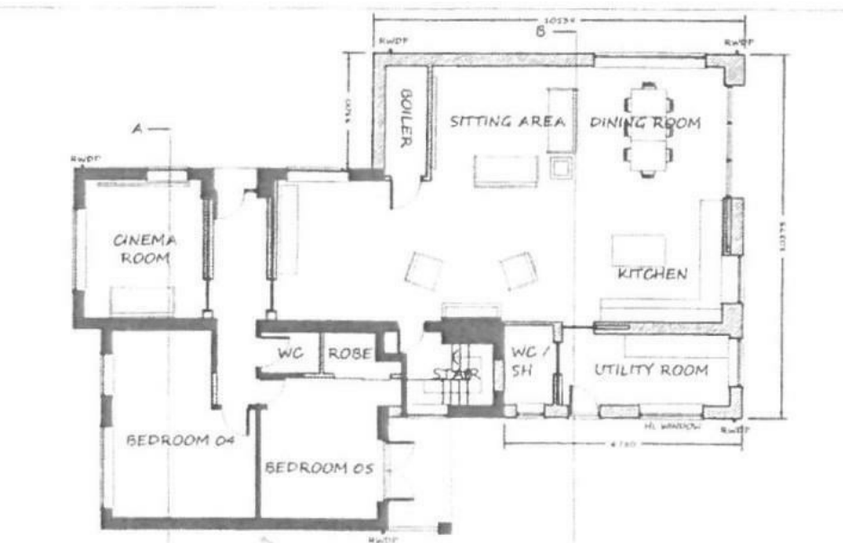
GROUND FLOOR PLAN AS PROPOSED
